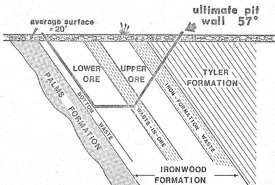
Penoque Range iron ore deposit and potential pit design. 10
